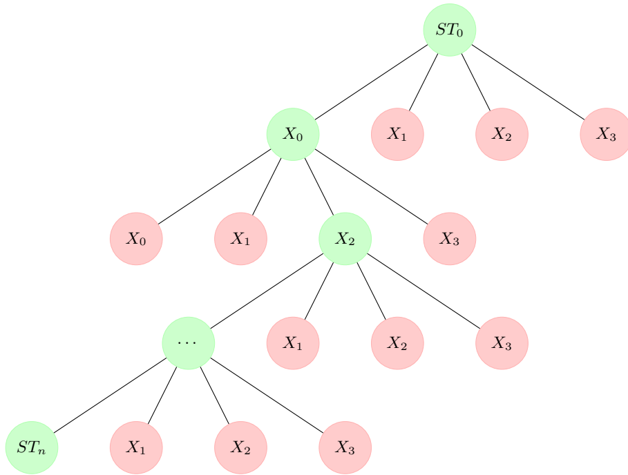
FIGURE 5 – Preimage tree in the Rabin function.
