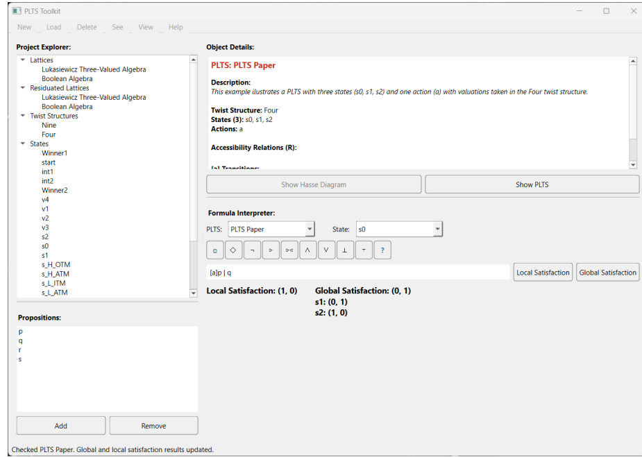
Fig. 4. Screenshot of the PLTS toolkit.
