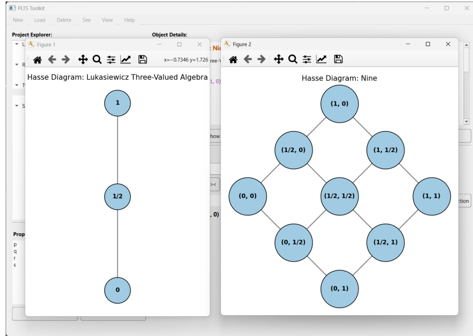
Fig. 5. Screenshot of the PLTS toolkit rendering of the Hasse diagram of 3 and \mathcal{NIN}\mathcal{E} .
