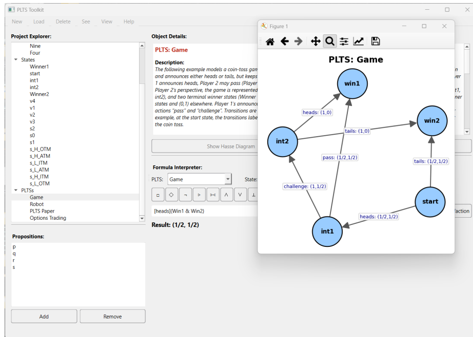
Fig. 7. Screenshot of the PLTS toolkit interpreting a formula for the PLTS in Figure 9.
