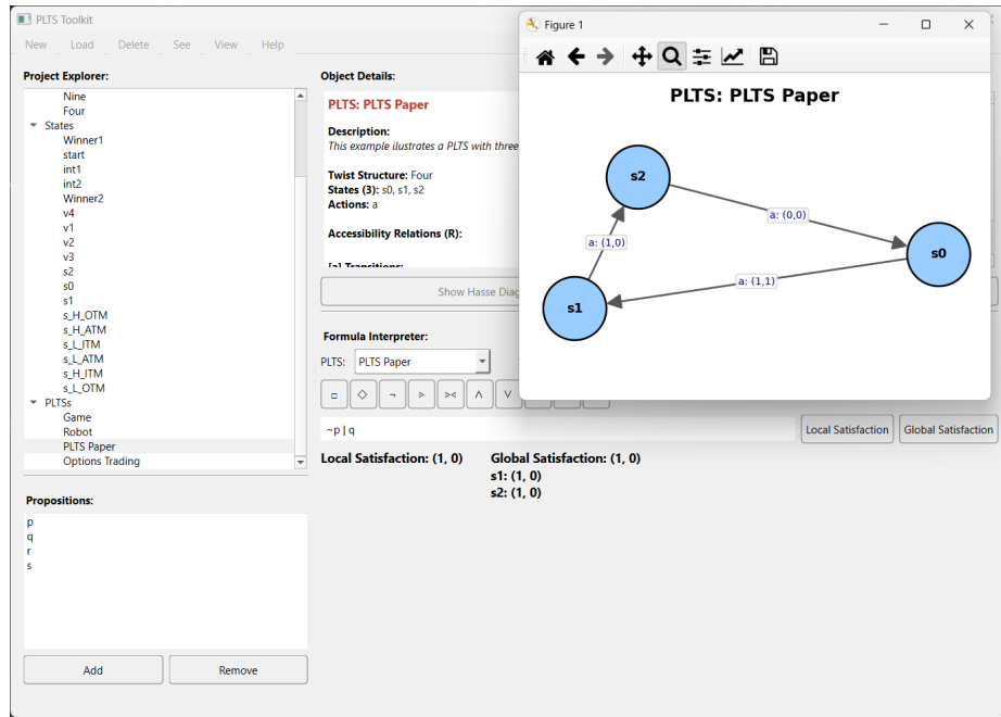
Fig. 6. Screenshot of the PLTS toolkit interpreting a formula for the PLTS in Figure 3.
