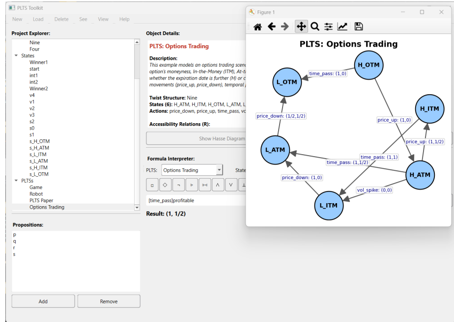
Fig. 11. Screenshot of the PLTS toolkit interpreting and checking the validity of formula for the PLTS in Figure 10.
