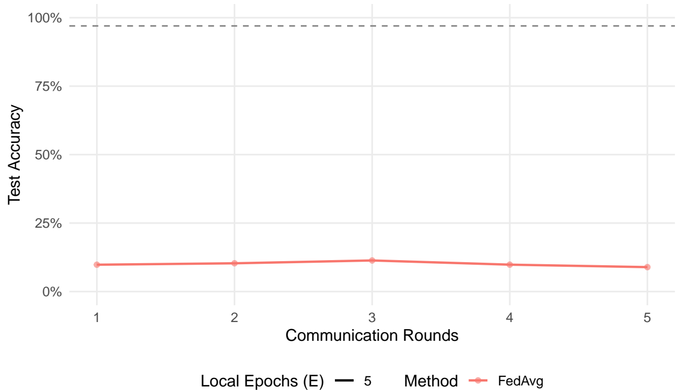
MNIST (Non-IID): Test Accuracy vs Communication Rounds
