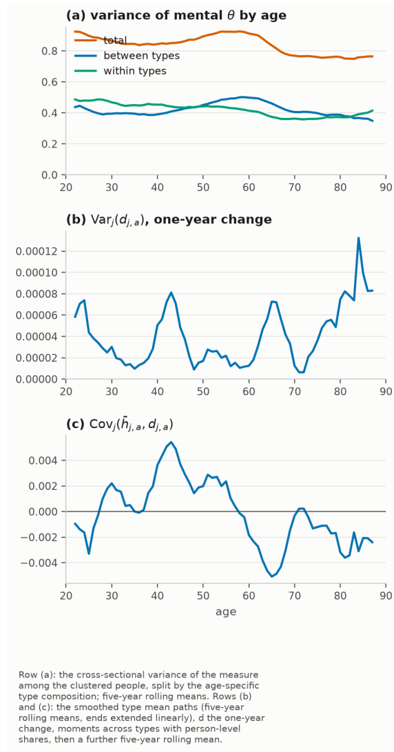
Figure H.34: As Figure 5, between versus within by age, on the mental GRM types.
