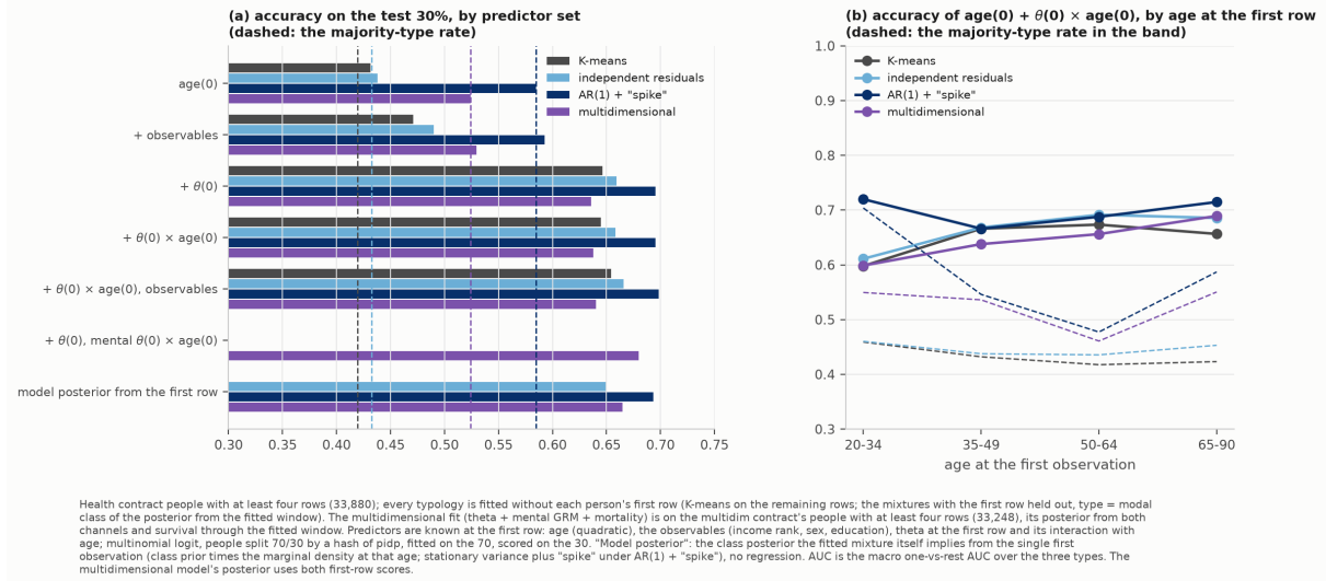
Figure 13: Predicting the type from a single initial observation, on \theta . Every typology is fitted without each person's first row (people with at least four rows, 33,880): partial K-means on the remaining rows, the independent-residuals and AR(1) plus "spike" mixtures with the first row held out, the type being the modal class of the posterior from the fitted window, and the multidimensional AR(1) plus "spike" fit with mortality likewise (on the multidimensional contract's people with at least four rows, 33,248; posterior from both channels and survival through the fitted window). (a) Accuracy on the test 30% by predictor set, multinomial logit on what is known at the first row; dashed, the majority-type rate. "Model posterior": the class posterior the fitted mixture itself implies from the one observation, no regression. (b) The same accuracy by age at the first observation.
