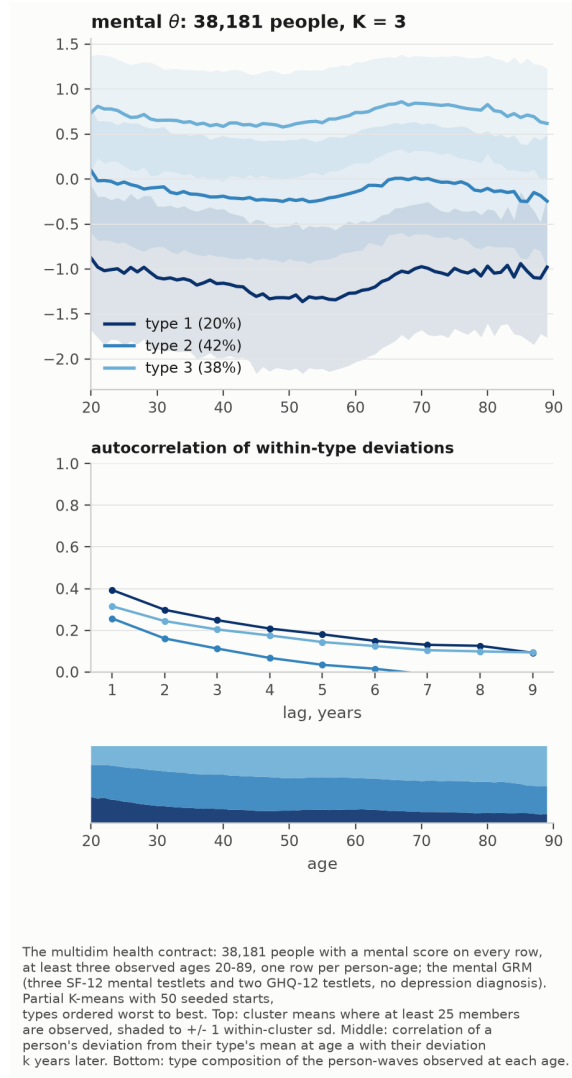
Figure H.33: As Figure 4, partial K-means types ( K = 3 ) on the mental GRM, on the multidimensional contract's rows.
