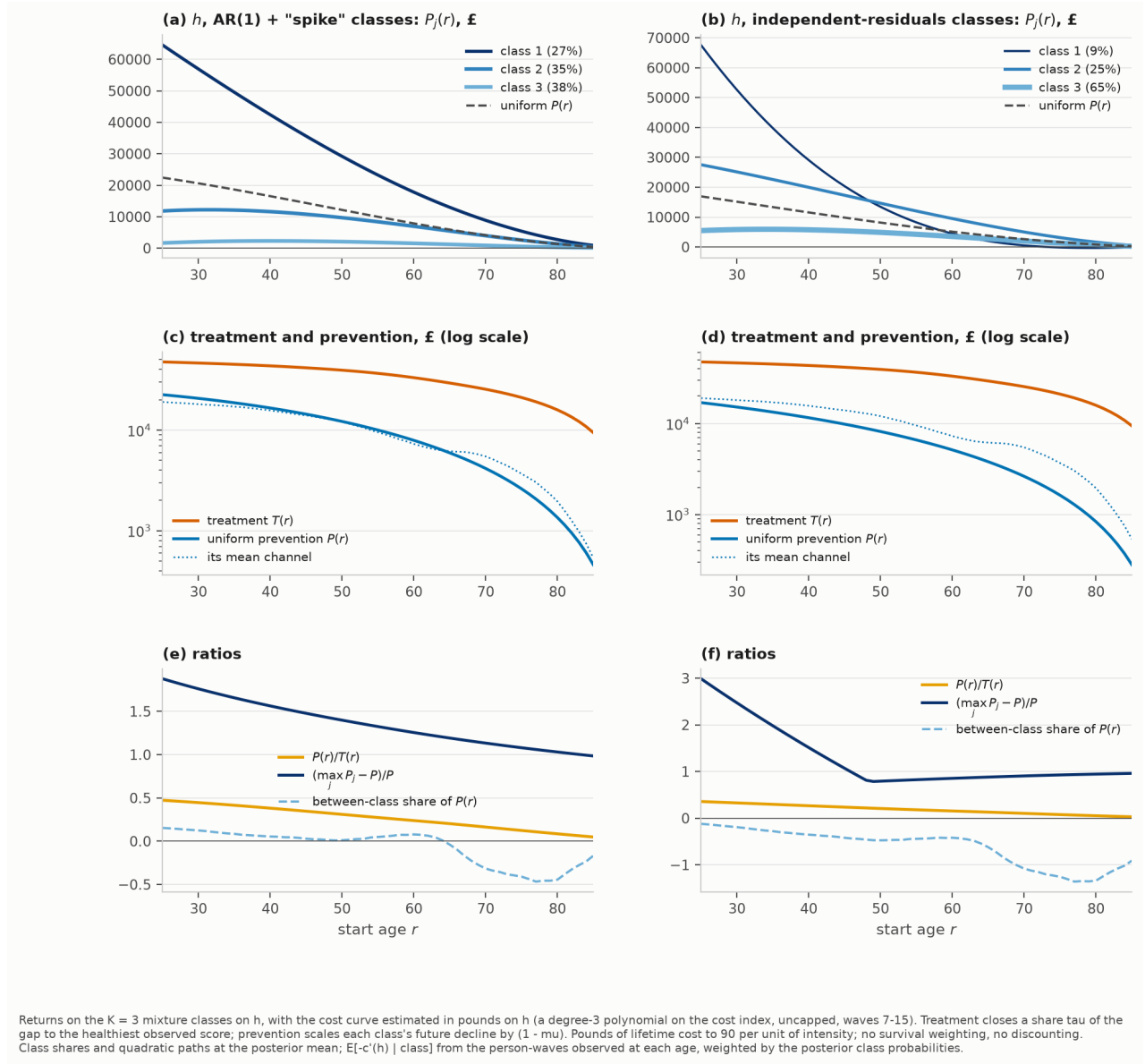
Figure C.17: As Figure 14, on h , with the cost curve estimated on h .
