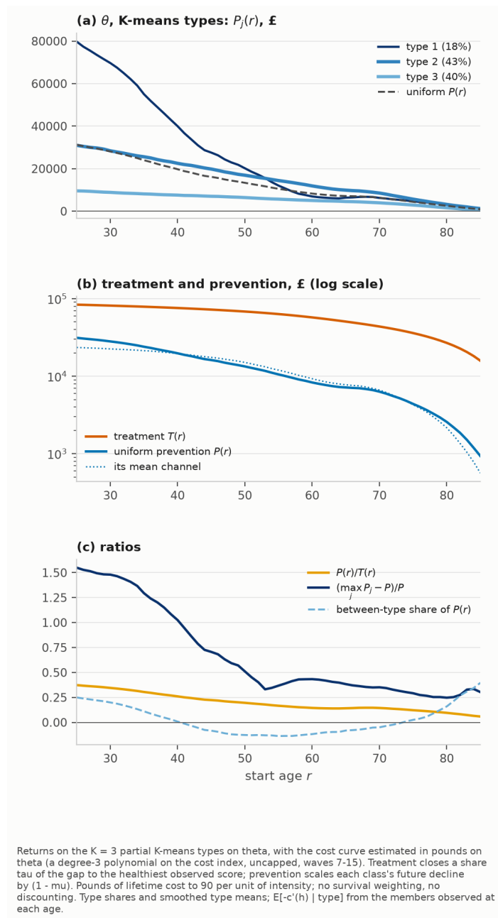
Figure G.28: As Figure 14, on the partial K-means types on \theta : type shares and smoothed type means, with the same uncapped cost curve.
