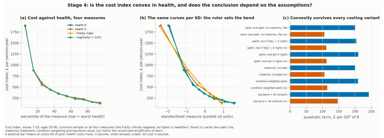
Figure B.2: Cost index in pounds against the four health measures ( \theta , h , and the frailty index and log frailty negated): by decile, per standard deviation of each measure, and the sensitivity of the convexity to every costing assumption the index rests on. Measures oriented so higher means better health. Panel (c) varies the spell rule, maternity treatment, condition weighting and top-band value, each with a winsorised-at-the-99th-percentile twin.
