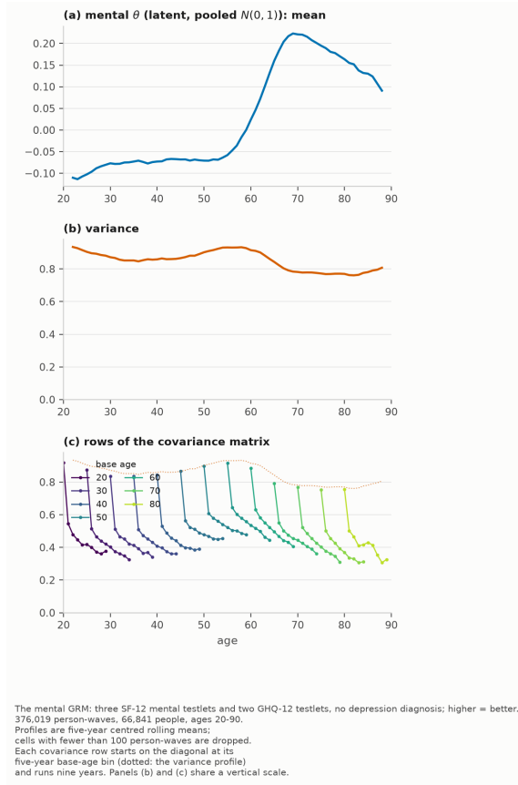
Figure H.31: As Figure 2, on the mental GRM: mean path, variance profile and covariance rows, model-free.
