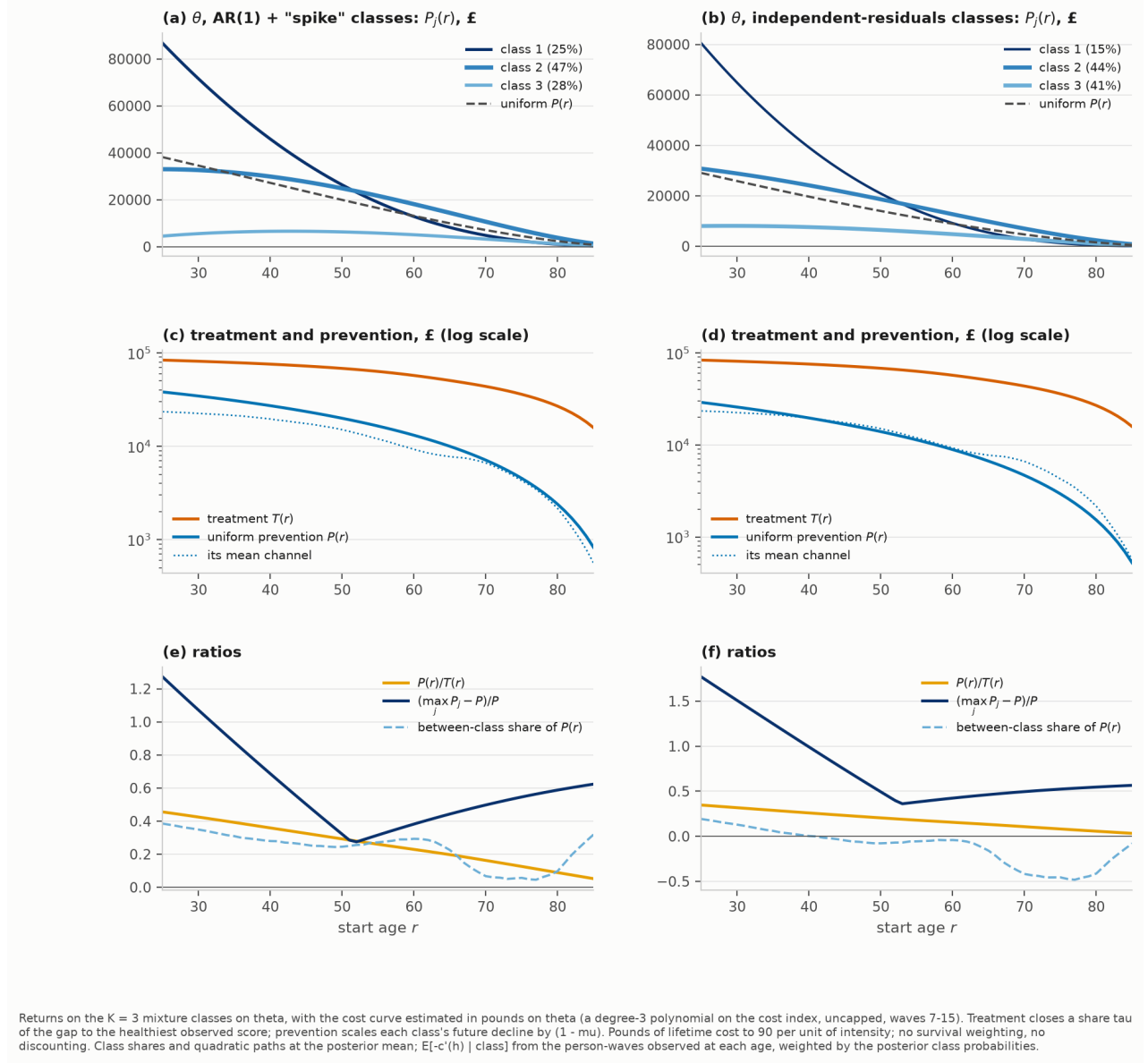
Figure 14: Returns to prevention and treatment by start age r on \theta , in pounds of lifetime cost under the estimated cost curve: (left) the AR(1) plus “spike” classes, (right) the independent-residuals classes. Top: P_j(r) by class and the uniform P(r) ; middle: T(r) , P(r) and its mean channel (log scale); bottom: P/T , the gain from class targeting relative to the uniform return, and the between-class share of P(r) .
