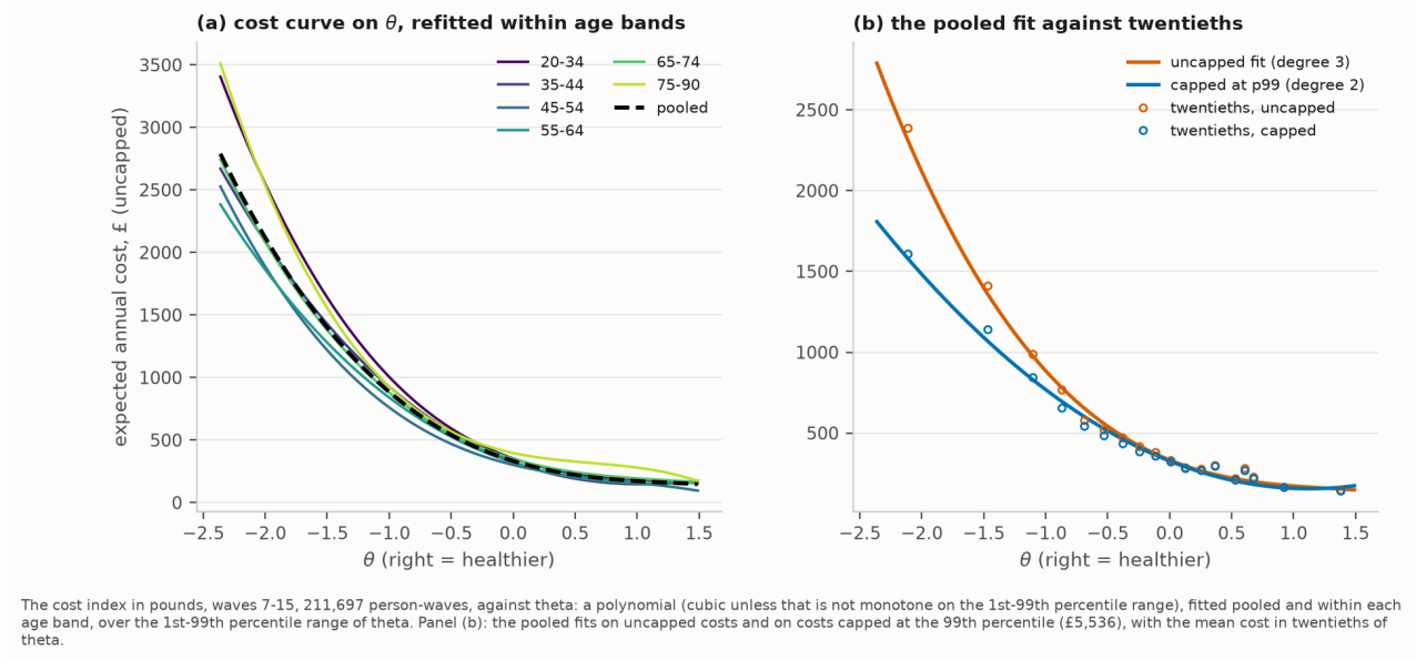
Figure G.27: The cost curve Section 5 prices with: the cost index in pounds against \theta , a cubic fitted to uncapped costs. (a) The same polynomial refitted within six age bands against the pooled fit; (b) the pooled fit on uncapped costs and on costs capped at the 99th percentile, against the mean cost in twentieths of \theta .
