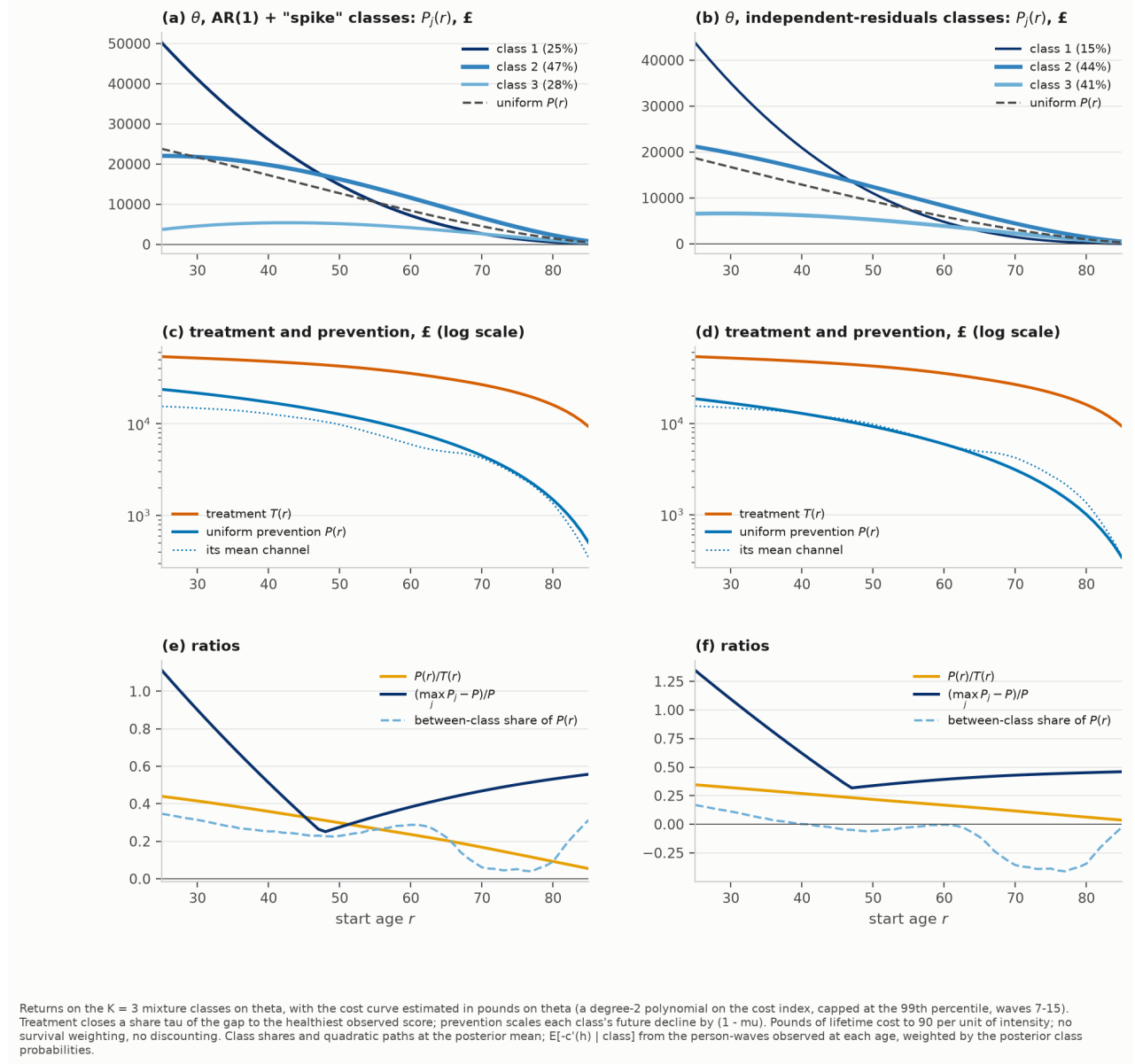
Figure G.29: As Figure 14, with the cost curve fitted to costs capped at the 99th percentile.
