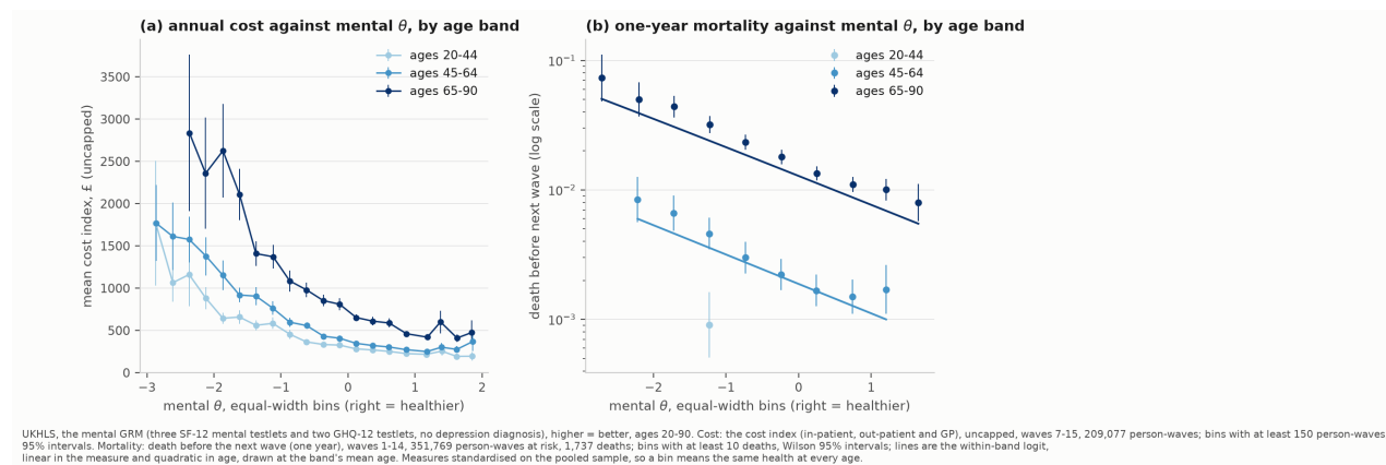
Figure H.30: As Figure 1, on the mental GRM.
