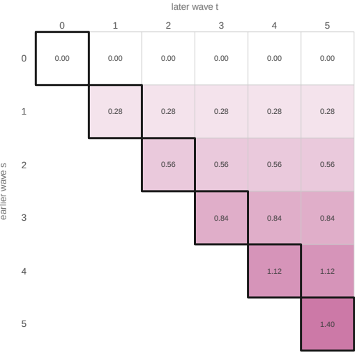
staircase: G(\min(s, t))
