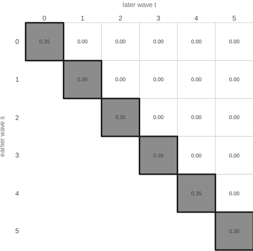
diagonal spike: \sigma_e^2
