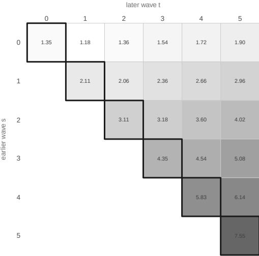
the matrix: sum of the five
