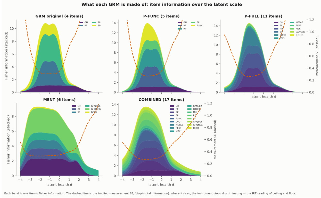
Figure 1: What each GRM is made of: stacked item information over the latent scale, with the implied measurement SE (dashed, right axis); each band is one item, ordered as in the legend. Panels: GRM original is the four-testlet physical measure replicated from the EIT note; P-FUNC adds the functioning testlet; P-FULL adds the six diagnosis groups; MENT is the mental bank; COMBINED is all seventeen items at once. Physical items, from the SF-12: GH general health (the single self-rated-health question), PF physical functioning (moderate activities, climbing stairs), RP role-physical (cutting down or being limited at work because of physical health), BP bodily pain; FUNC is the count of Equality Act physical limitations (mobility, lifting, dexterity, coordination, personal care). Diagnosis groups: CVD cardiovascular events, METAB diabetes and high blood pressure, RESP chronic airway disease, MSK arthritis, CANCER , OTHER the pooled remainder of thyroid, liver and epilepsy (§2.3). Mental items: MH mental health (calm; downhearted), RE role-emotional (cutting down or working less carefully because of emotional health), SF social functioning (health interfering with social activities), GHQPOS and GHQNEG the positively- and negatively-worded halves of the GHQ-12, DEPR ever-diagnosed clinical depression. FUNC adds a broad band of precision on the ill side; the condition items are visibly thin; GHQ-negative dominates the mental bank; the combined bank is tallest and widest but its SE still rises sharply above \theta \approx +1 .
