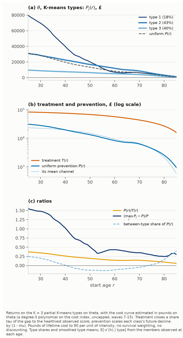
Figure G.28: As Figure 13, on the partial K-means types on \theta : type shares and smoothed type means, with the same uncapped cost curve.
