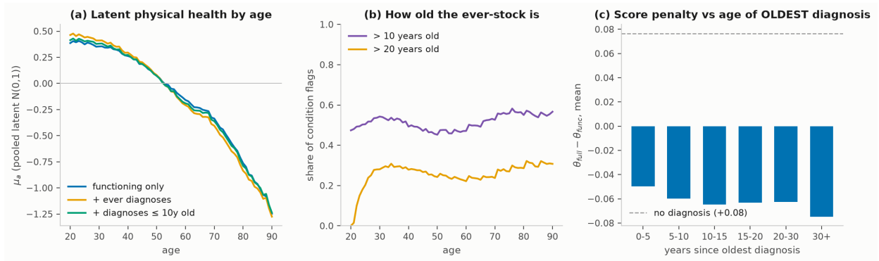
Figure 4: (a) latent age profiles with and without diagnoses and with only recent diagnoses; (b) the staleness of the ever-stock; (c) the score penalty against the age of the oldest diagnosis.
