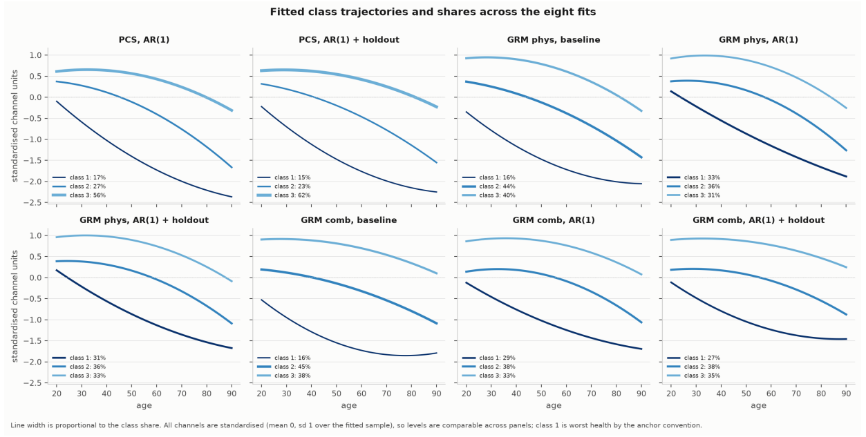
Figure 7: Fitted class mean trajectories \alpha_k + \beta_k a + \gamma_k a^2 (with a = (\text{age} - 55)/10 ) for all eight fits, on each channel's standardised scale. Line width is proportional to the class share.
