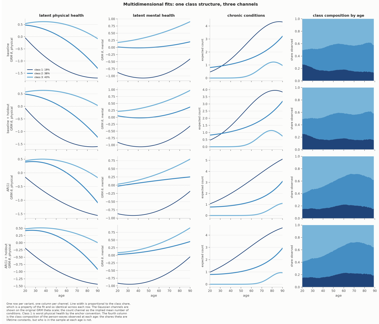
Figure 9: Class trajectories and shares for the four multidimensional fits, one row per variant and one column per channel. A fit has a single class structure, so the shares are identical across a row and the line width (proportional to the share) repeats; what changes across the row is what each class does on each channel. The Gaussian channels are returned to the original GRM \theta scale using each fit's standardising moments; the count channel shows the implied mean number of conditions. Class 1 is worst physical health by the anchor convention. Together with Figure 8, which covers the eight univariate fits, every Bayesian model in this note has its trajectories and shares drawn.
