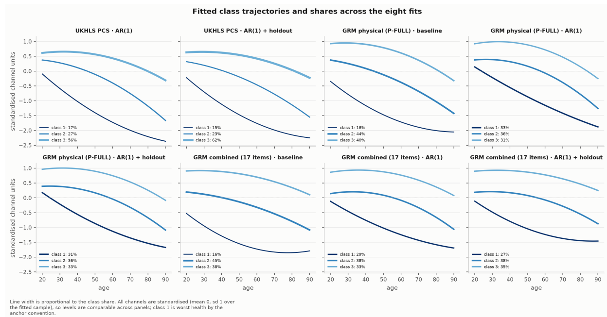
Figure 8: Fitted class mean trajectories \alpha_k + \beta_k a + \gamma_k a^2 (with a = (\text{age} - 55)/10 ) for all eight fits, on each channel’s standardised scale. Channels: the UKHLS PCS, the physical GRM in its P-FULL specification ( theta.phys.full : functioning plus diagnosis groups), and the combined seventeen-item GRM ( theta.combined ). Line width is proportional to the class share.
