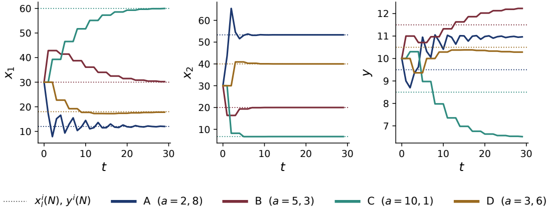
Figure 4: Dynamics of allocations with multiple goods. The dotted lines are the centralised benchmarks x_l^i(N) and y^i(N) .
