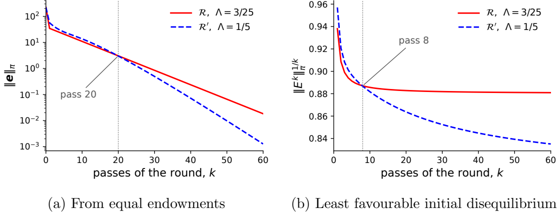
Figure 8: Convergence of the two rounds of Example 11, against the number of passes k of each round. A pass of \mathcal{R} has two trades and a pass of \mathcal{R}' has three. Panel (a) shows \|e\|_\pi after k passes from the equal-endowment profile \omega^i = 36 , on a logarithmic scale. Panel (b) shows \|E^k\|_\pi^{1/k} , the largest share of disequilibrium that can remain after k passes, expressed per pass.
