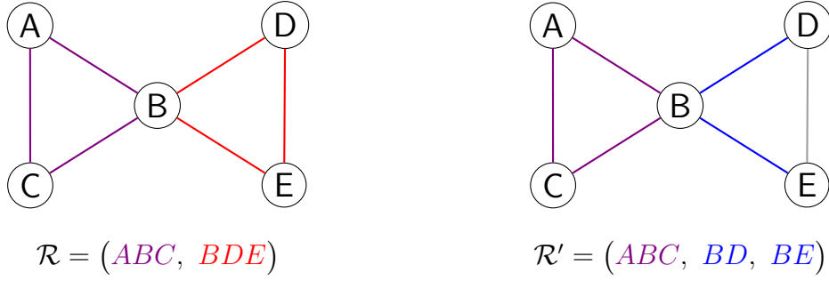
Figure 7: The two rounds of Example 11 on the bowtie. Red marks the coalition that only \mathcal{R} convenes, blue the coalitions that only \mathcal{R}' convenes, and purple the coalition ABC that both convene. The colours match Figure 8. The two rounds differ only in the link DE , which the refinement leaves unused.
