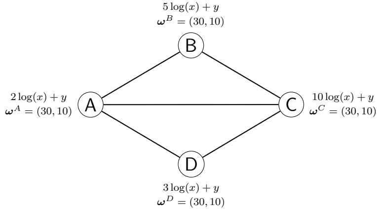
Figure 5: The diamond network of Example 5. The two triangles are ABC and ACD , and agents A and C belong to both.
