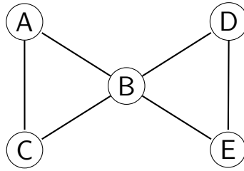
Figure 6: The bowtie network of Example 10. The two triangles are the largest coalitions available, and agent B is the only agent belonging to both.
