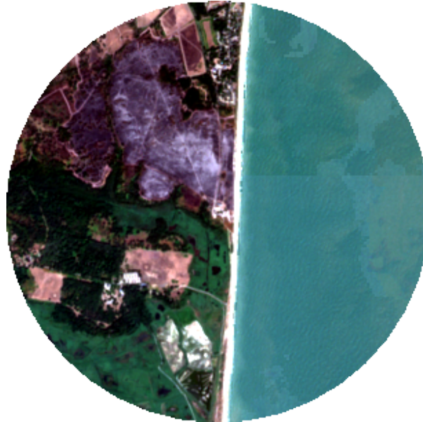
Burn severity
