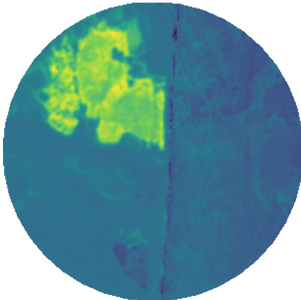
Difference NBR
