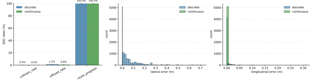
Figure 9: Effect of action discretization on inferred-expert-action quality. We replay each agent’s logged trajectory through the simulator using actions inferred from the logs, comparing discrete (bin-quantized, blue) and continuous (direct float, green) action representations. Left: SDC rates aggregated across 10,240 pooled samples; both representations complete the route in 100% of scenarios, but discretization induces modestly higher off-road and collision rates. Center, right: distributions of per-trajectory lateral and longitudinal L2 error to the logged pose. Continuous actions reproduce the log almost exactly (errors concentrated near zero), while discrete actions exhibit a small but consistent quantization floor of \sim 0.1 m laterally. Error bars on the bar plot denote standard error.
