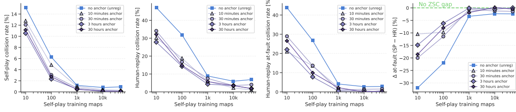
Figure 4: Scaling laws for scenario metadata. The unregularized self-play baseline is shown in blue; shades of purple correspond to regularized policies trained with different BC anchors, with darker shades indicating more anchor data. Left: collision rate in self-play, where all agents are controlled by the same policy on a held-out validation set. Center left: collision rate in human-replay, where only the SDC is controlled and the remaining agents follow their logged trajectories. Center right: at-fault collision rate, the fraction of collisions caused by the controlled agent. This metric is more informative than raw collision rate, because replay agents frequently strike the SDC from behind, and such collisions would be unlikely in practice (See cartoon in Figure 2). Right: ZSC gap \Delta_{ZSC} , the difference in score between the self-play and human-replay settings.
