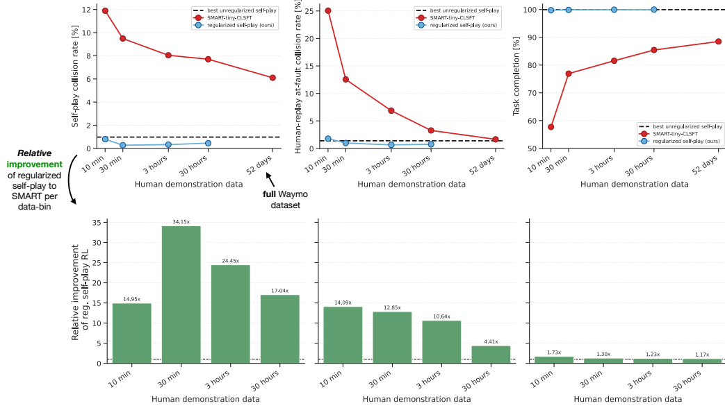
Figure 3: Scaling laws for human demonstration data. Performance of regularized self-play RL (—●—) and SMART with CAT-K closed-loop fine-tuning (—●—) as a function of the amount of human demonstration data used for training, evaluated in self-play and against human replays. All policies are evaluated on the same 10k held-out scenarios from the Waymo Open validation set [23]. Regularized self-play saturates at roughly three hours of human data, whereas SMART continues to improve across the full WOMB training set. Self-play RL (---) is shown as a horizontal line, since it uses no human demonstrations. The horizontal axis is semi-logarithmic.
