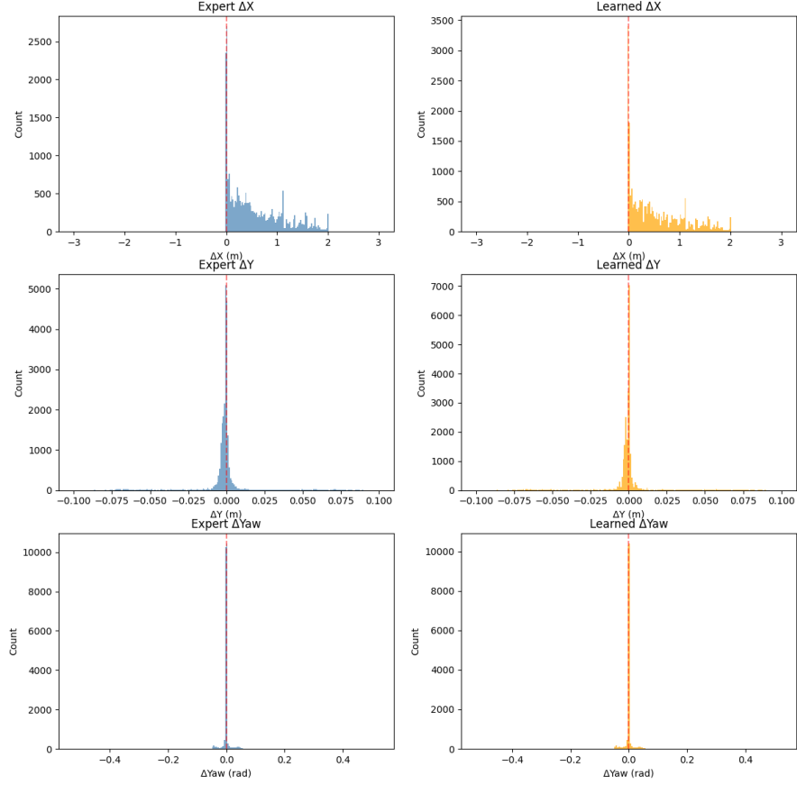
BC Training Data vs Learned Policy — 23296 samples, delta_local, 67 maps
