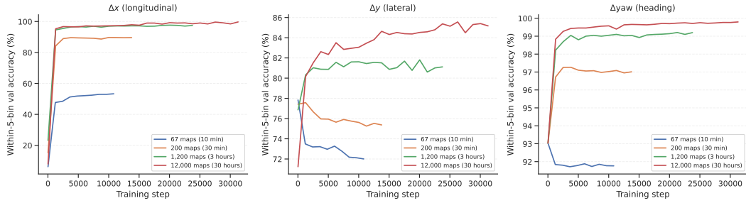
Figure 12: Training curves for the anchor policies. Each panel shows within-5-bin validation accuracy on a held-out set of scenarios for one action component ( \Delta x , \Delta y , \Delta \psi ). Curves terminate at different step counts because training stops once validation accuracy plateaus (no improvement for 100 consecutive epochs).
