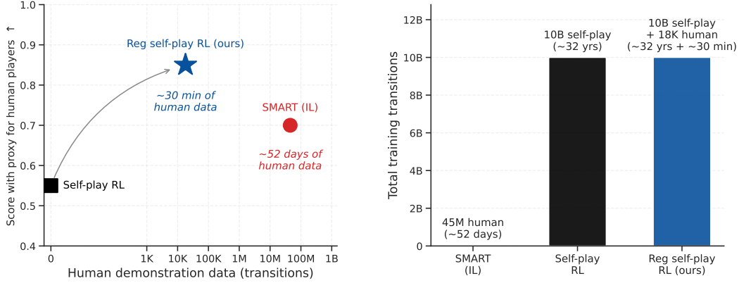
Figure 1: TODO Regularized self-play RL reduces the human-coordination gap with a pinch of human demonstration data. Left: score on a human-replay evaluation (proxy for human-compatibility) versus human demonstration data per method. Adding 30 min of human demonstrations as an RL anchor (star, ours) increases performance well above the unregularized self-play baseline (square) and SMART (circle), an imitation-learning model trained on the full Waymo dataset. Right: total training transitions per method. Our method is trained on substantially more data than SMART, which explains the performance improvement. However, in contrast to SMART, we train almost entirely on cheap synthetic data, whereas SMART trains on 45M human demonstration transitions (52 days).
