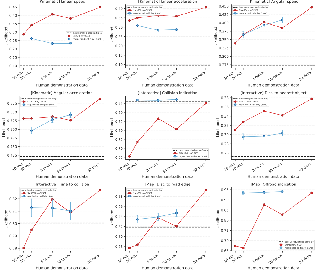
Figure 6: Submetrics
