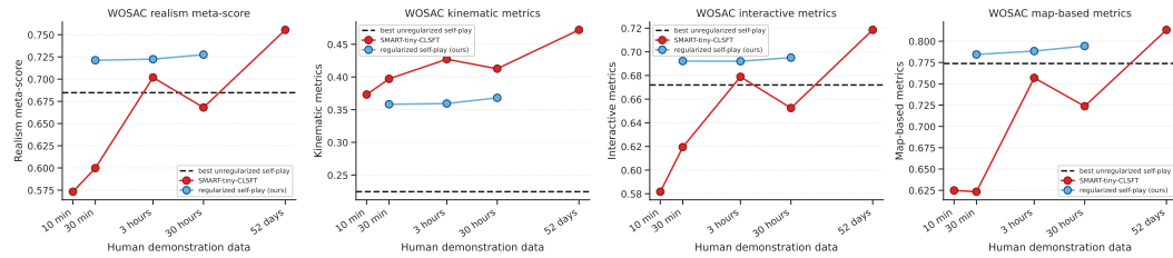
Figure 5: Enter Caption
