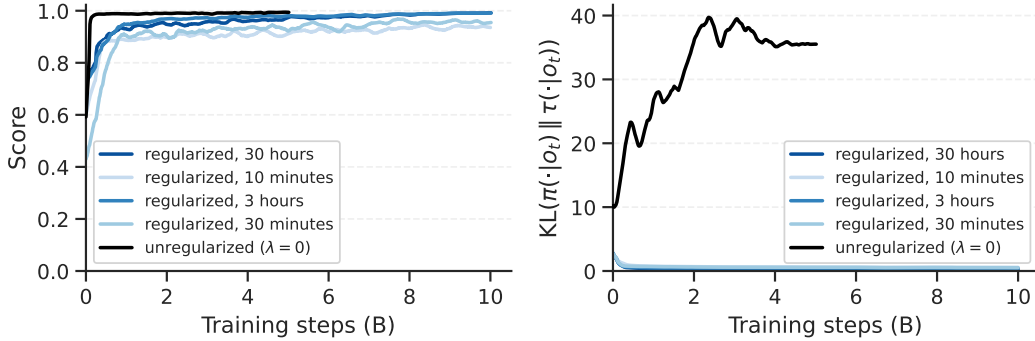
Figure 7: Regularized self-play policies stay close to the anchor distribution while unregularized self-play diverges. Here we show that, while both unregularized (black) and regularized self-play policies converge to effective strategies (left), the action distribution underlying these strategies varies widely as indicated by the kl divergence between the observation-conditioned action distributions (right). The regularized self-play policies stay close to the anchors, whereas the unregularized policies diverge.
