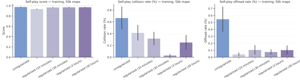
Figure 17: Performance of the policies trained on 50k maps on the full train dataset.
