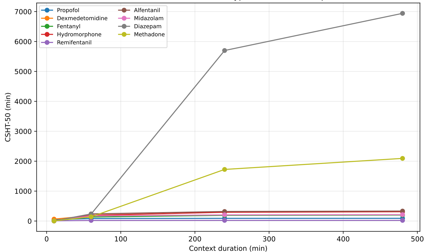
Plasma CSHT-50 vs Context (Hypnotics/Sedatives/Opioids)
