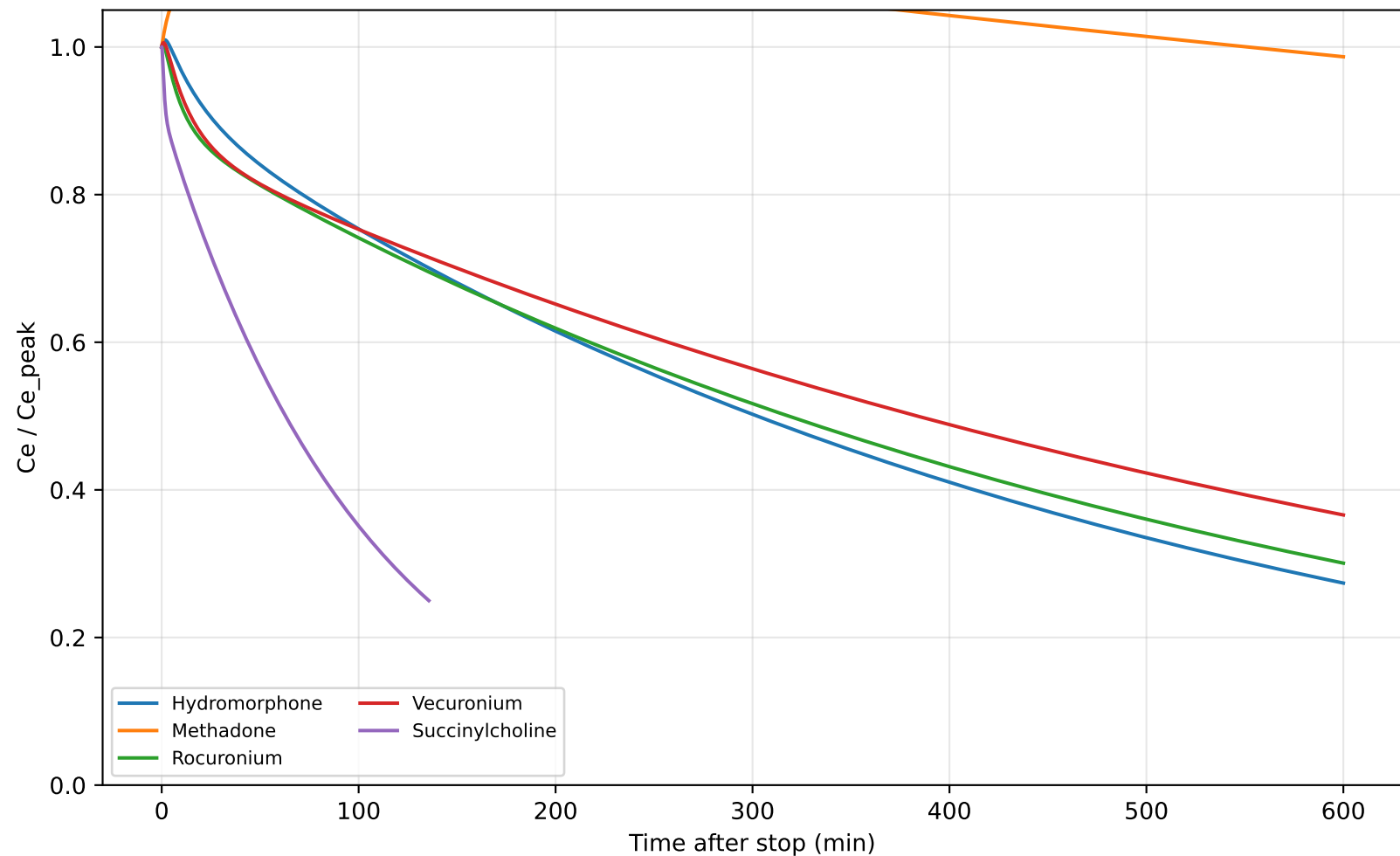
Effect-site Decrement (Normalized Ce) after 1h Context
