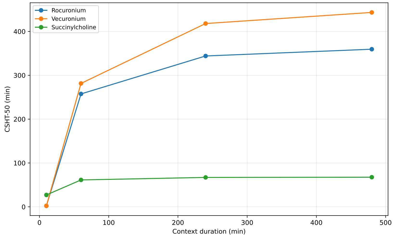
Plasma CSHT-50 vs Context (NMBAs)
