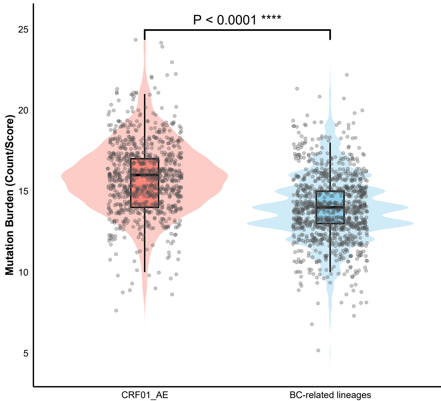
Figure 5: Lineage_Mutational_Burden(Track A)
