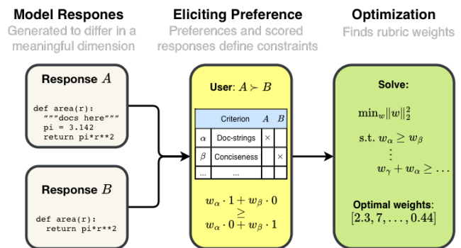
Fig. 1: Converting user preferences into optimized rubric weights.
