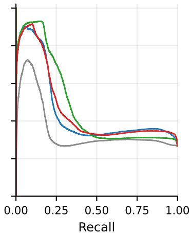
isolation forest
