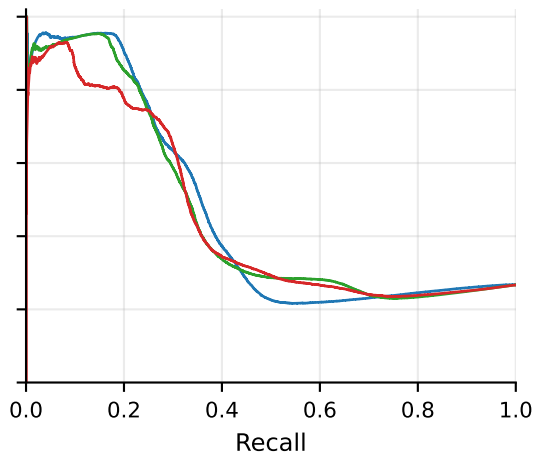
One-Class SVM
