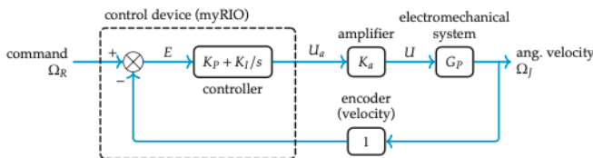
Figure 2: Control block diagram for the Lab 7 PI velocity-control system.
