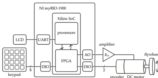
Figure 1: Schematic diagram of the target closed-loop system.
