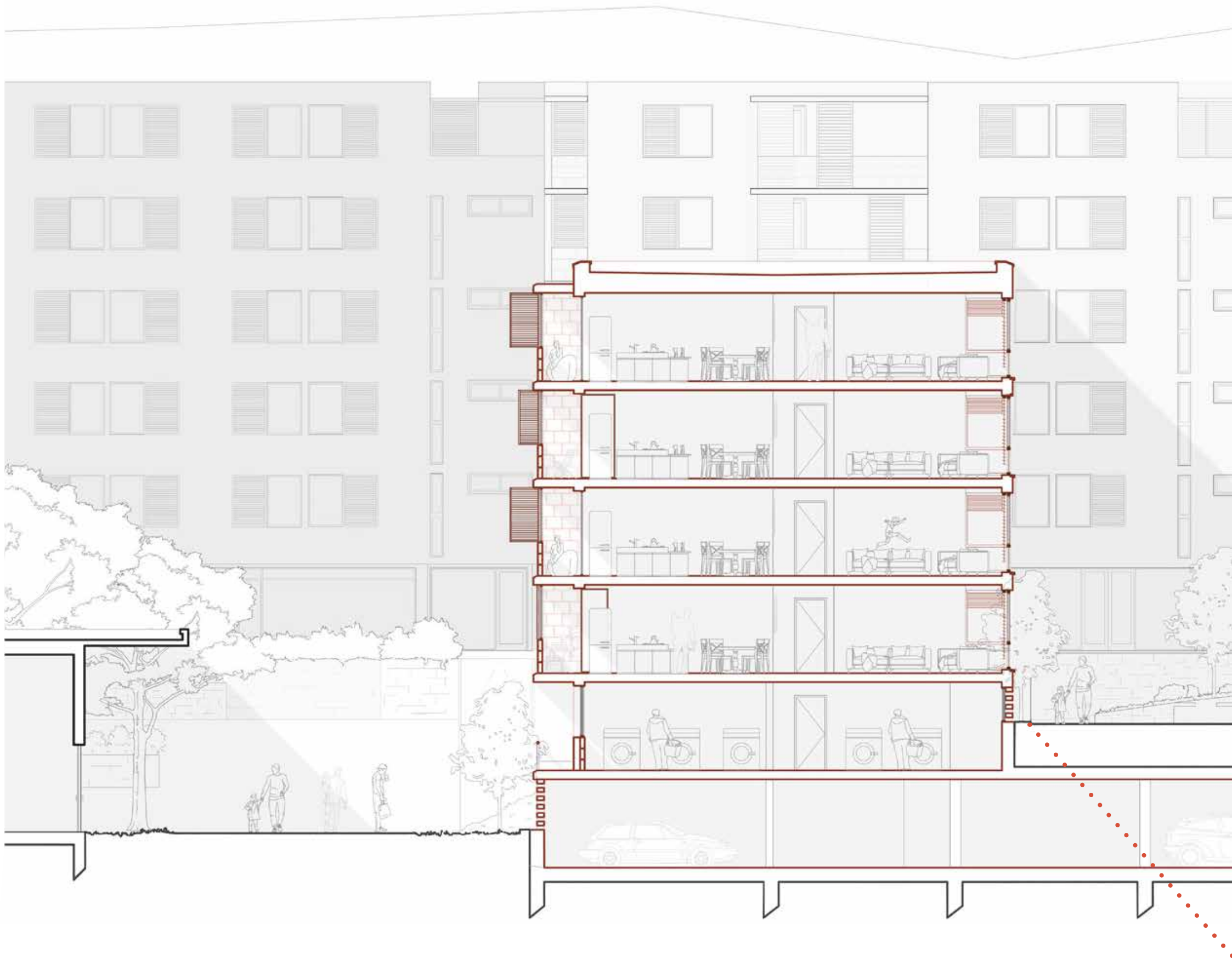
Site Section
