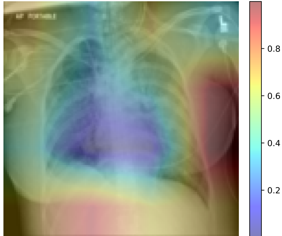
CAM
