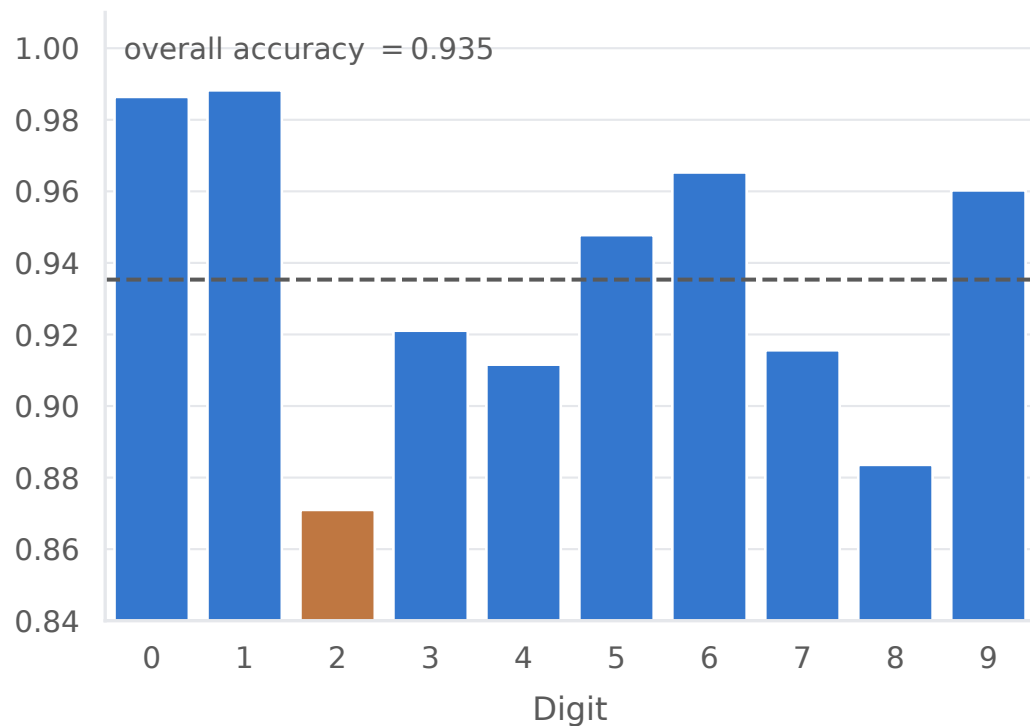
Per-class recall for k -NN
