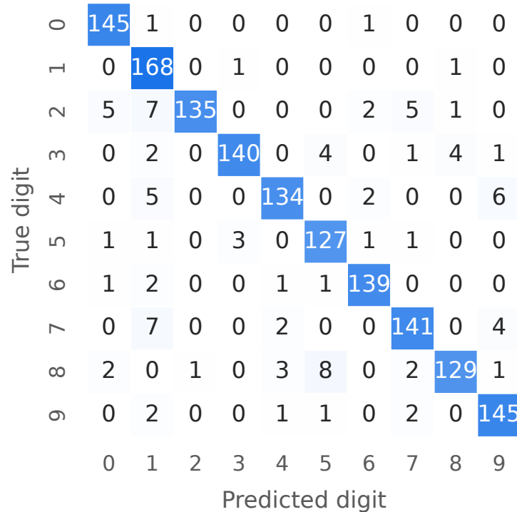
Confusion matrix on the held-out split
