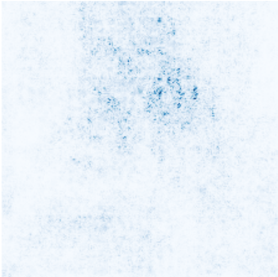
Saliency (Gradient)
