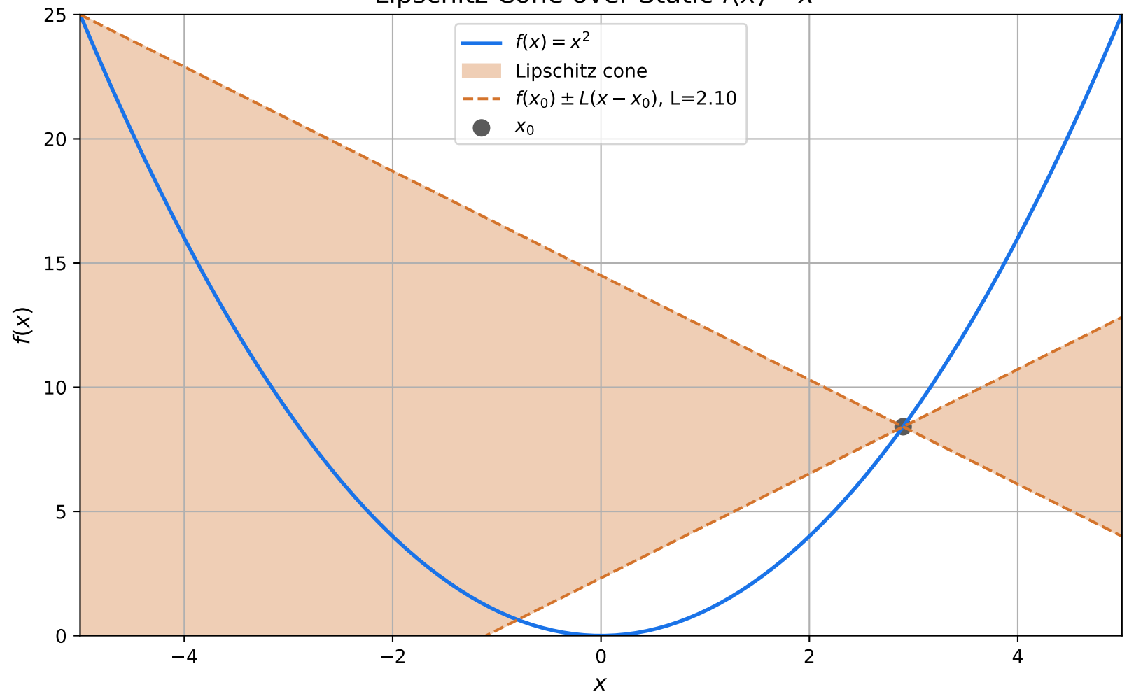
Lipschitz Cone over Static f(x) = x^2
