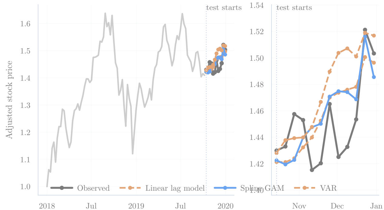
stock: full forecast
