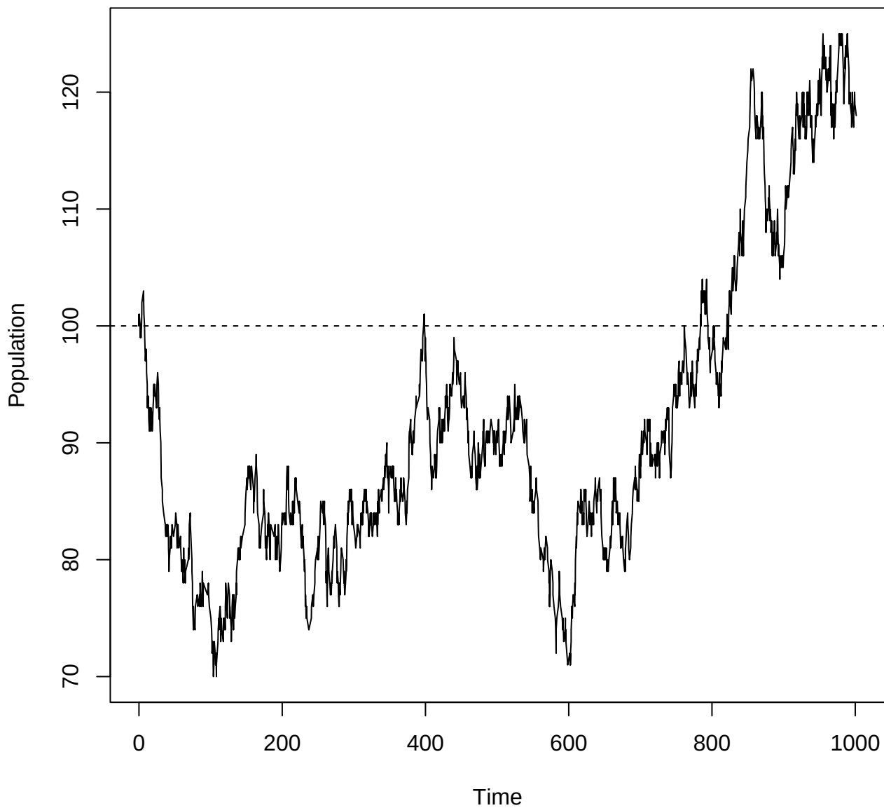
Birth-death process, b=0.01 , d=0.01
