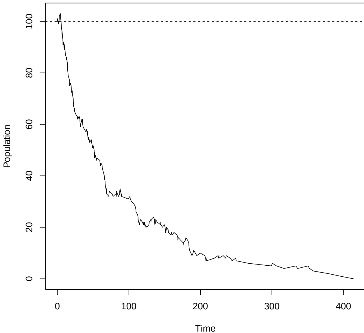
Birth-death process, b=0.01 , d=0.02
