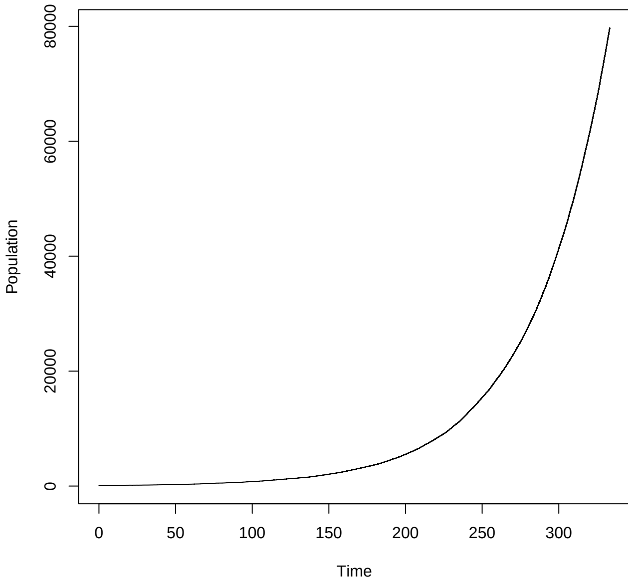
Birth-death process, b=0.03 , d=0.01
