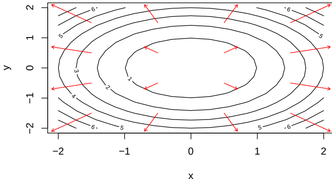
Gradient Field
