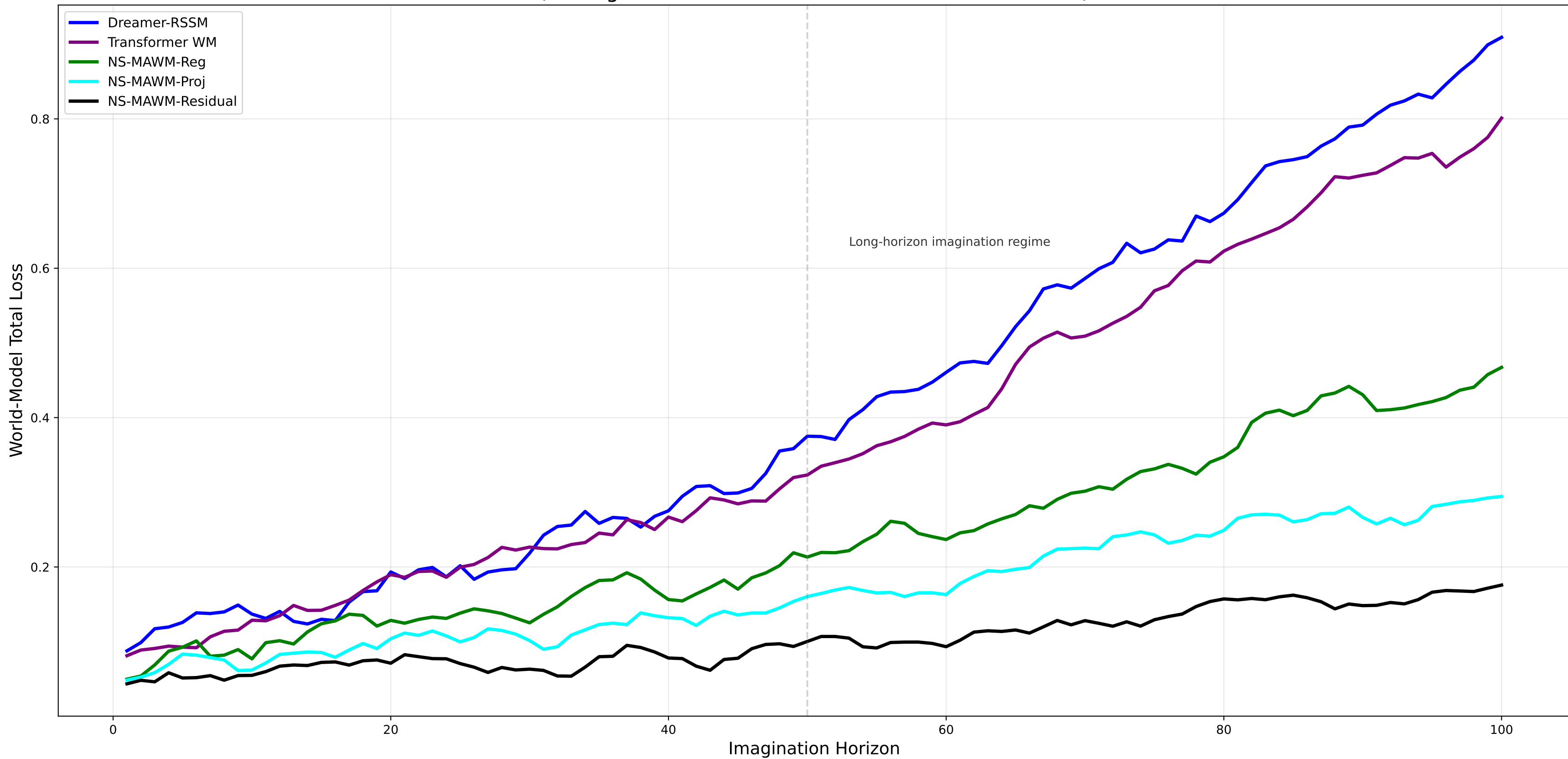
Compounding-Error Curves (Averaged and Smoothed Across Seeds and Variants)
