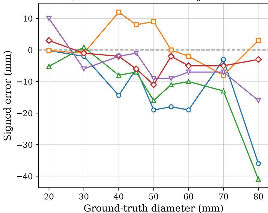
(b) Estimation error vs. object size
