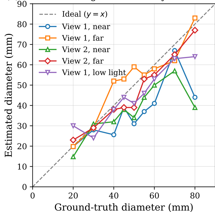
(a) Estimated vs. ground-truth cylinder diameter
