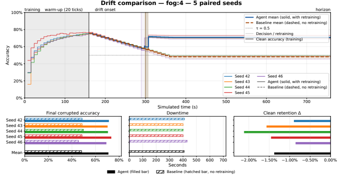
Fig. 1. Fog, 200s ramp, five paired seeds. Top: corrupted accuracy over simulated time (solid: reactive, dashed: baseline; thick lines: means); \tau = 0.5 dashed; shaded bands: the retraining round. Bottom: final corrupted accuracy, downtime, and clean retention; the reactive arm never falls below \tau (zero downtime).
