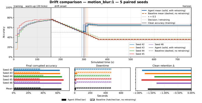
Fig. 2. Motion blur, 200s ramp, five paired seeds. The reactive arm recovers within one round and stays above \tau for most of the horizon; the baseline keeps degrading to about 0.35.
