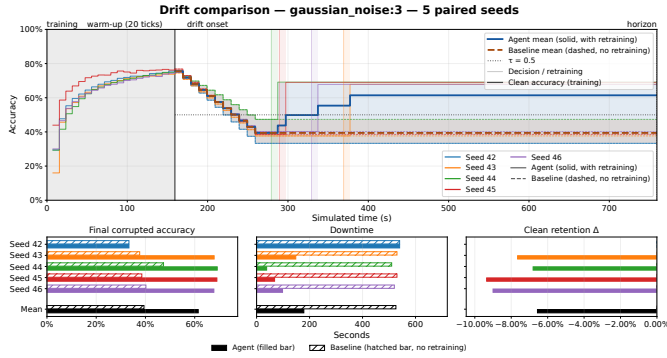
Fig. 3. Gaussian noise, 100s ramp, five paired seeds. Seed 42 never triggers. Its trajectory (solid blue) does not recover, while the other four seeds recover to about 0.68.
