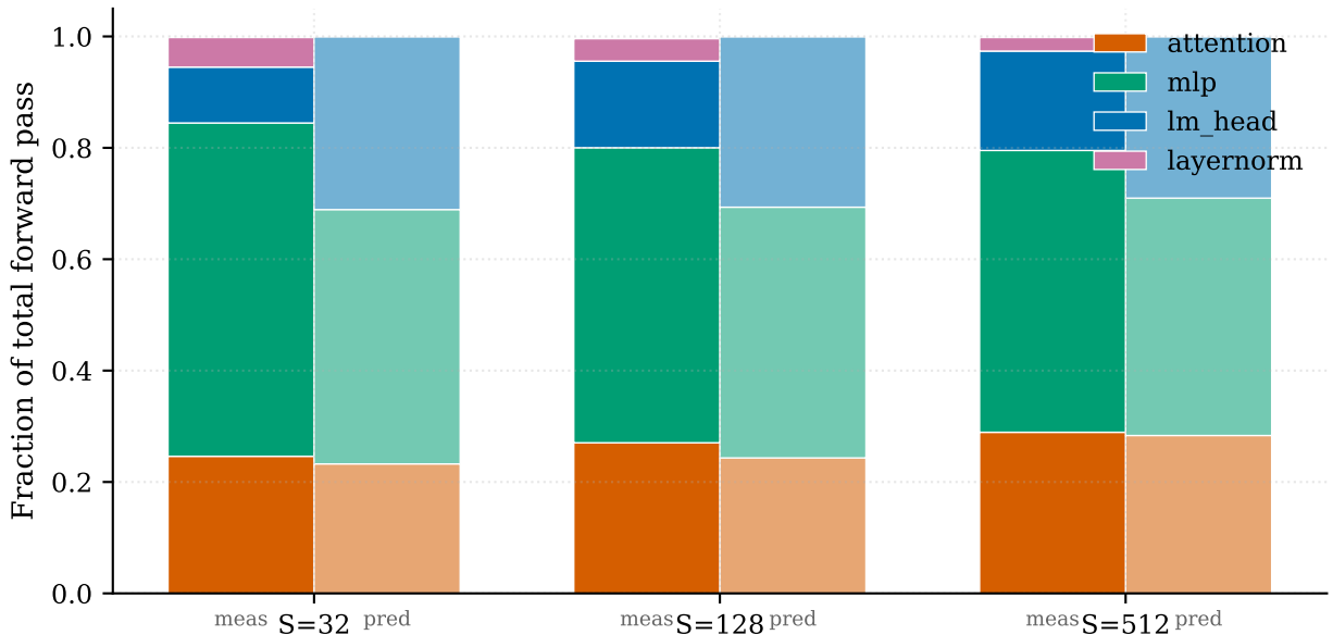
Time-share (measured) vs FLOP-share (predicted) by component
