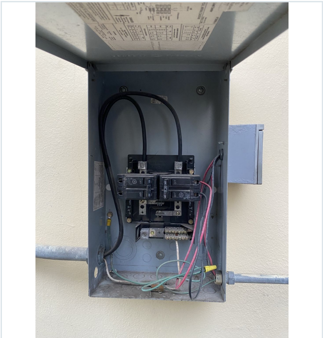
08 Electrical enclosure interior
