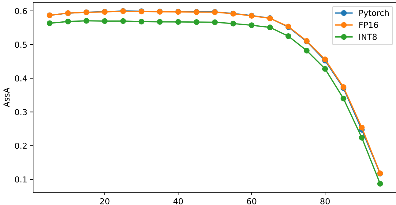
AssA vs IoU - Tracking1 (format)
