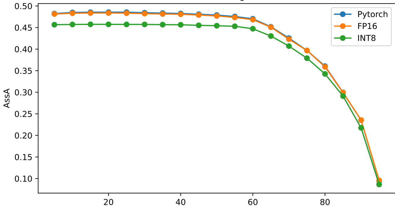
AssA vs IoU - Tracking2 (format)
