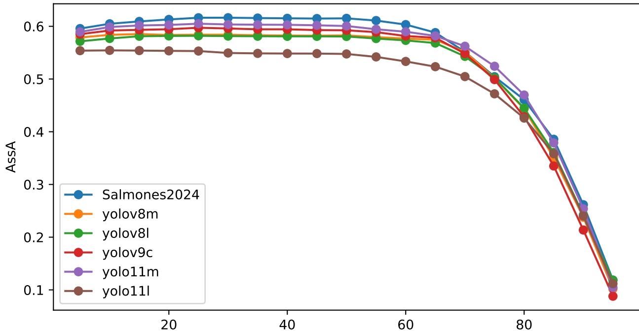
AssA vs IoU - Tracking1 (model)
