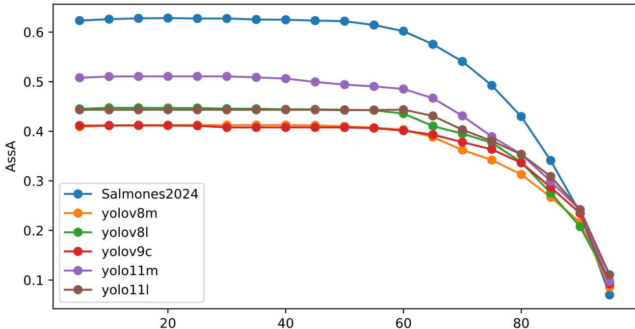
AssA vs IoU - Tracking2 (model)
