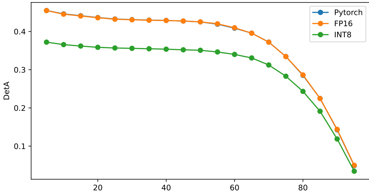
DetA vs IoU - Tracking1 (format)
