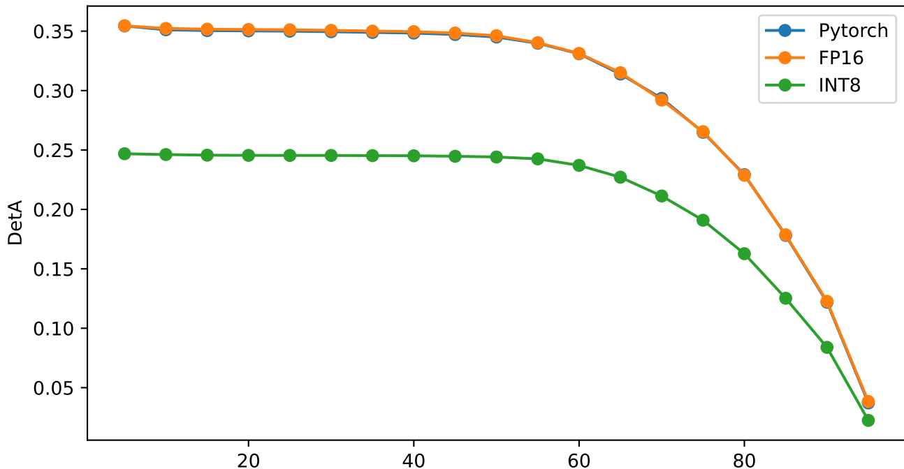
DetA vs IoU - Tracking2 (format)
