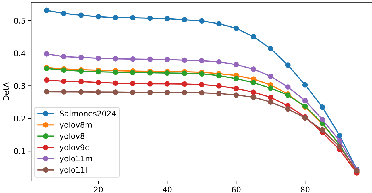
DetA vs IoU - Average (model)
