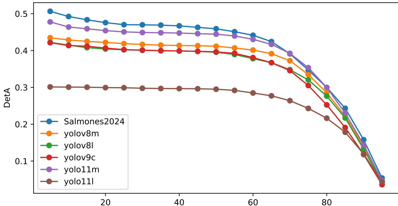
DetA vs IoU - Tracking1 (model)
