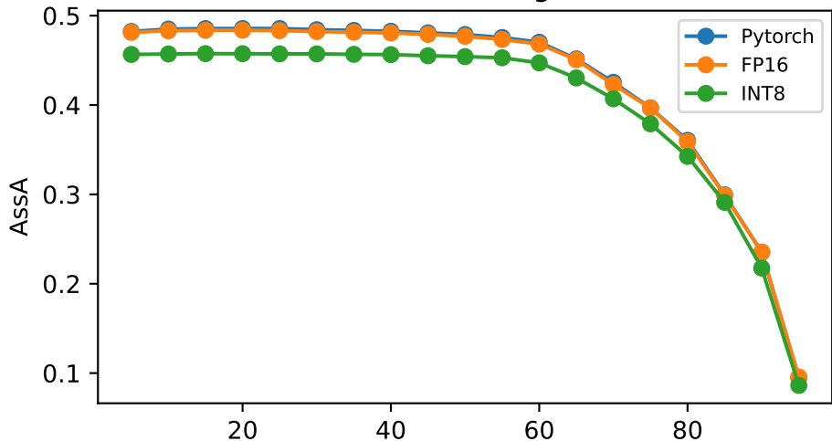
AssA vs IoU - Tracking2 (format)
