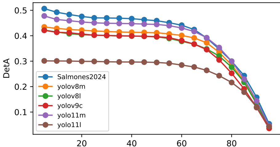
DetA vs IoU - Tracking1 (model)
