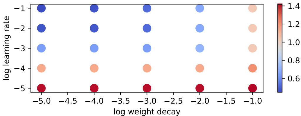
Validation loss
