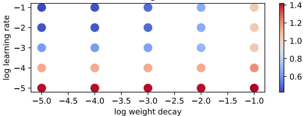
Validation loss
