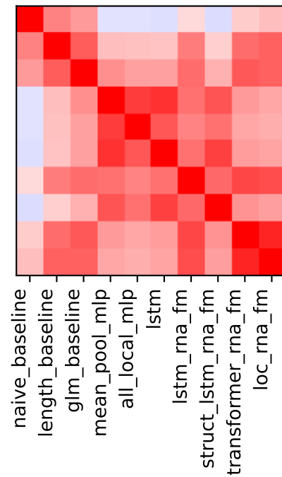
Wasserstein Distance
