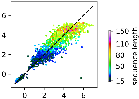
bilstm
