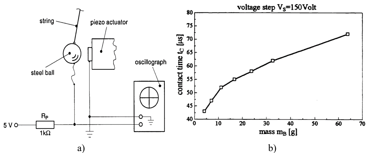
Figure 52 Left: Setup for measuring the contact time t_d ; right: contact time t_d as a function of the mass m_B (Images used with kind permission from Klaus Moldovan (Muth et al., 1995, p. 699) )
